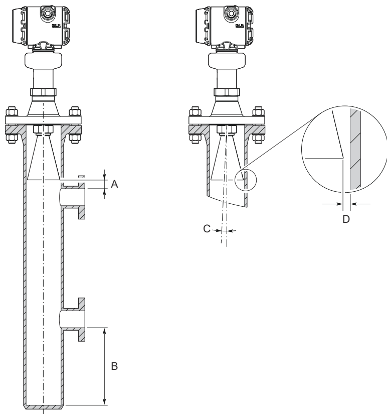
Figure 25: Chamber Requirements
