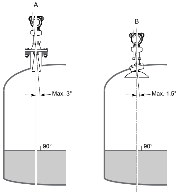
Figure 19: Inclination
