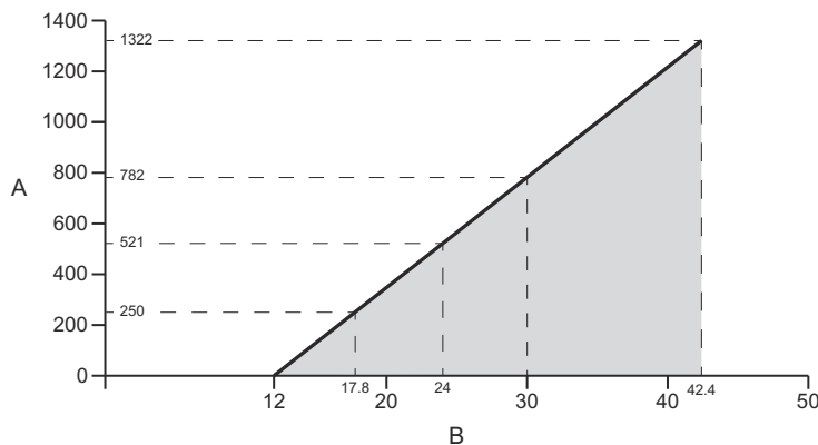
Figure 5: Load Limits
