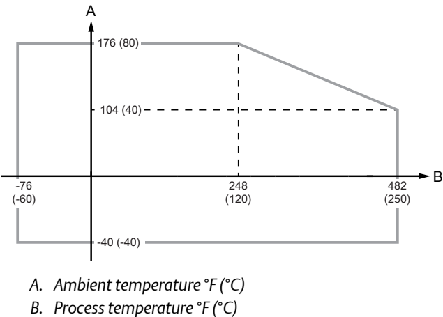
Figure 13: Ambient Temperature vs. Process Temperature
