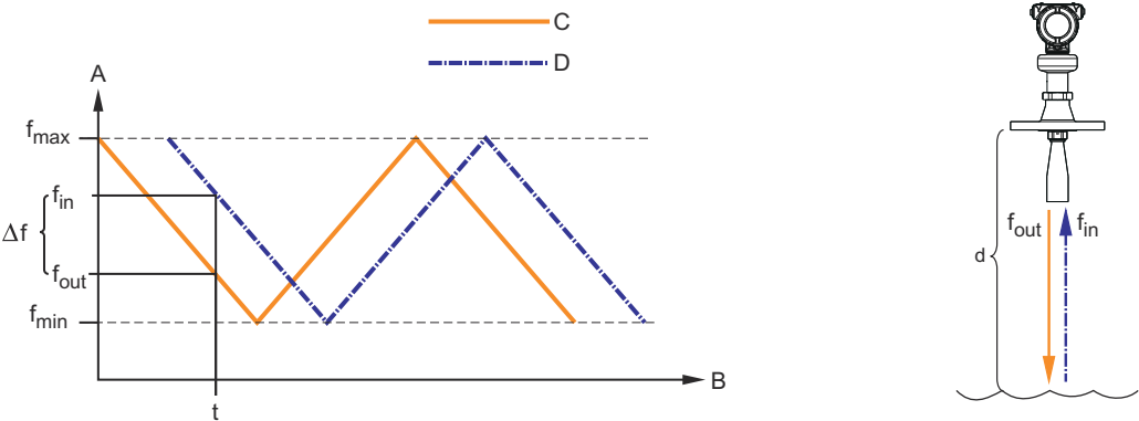
Figure 1: FMCW-method
